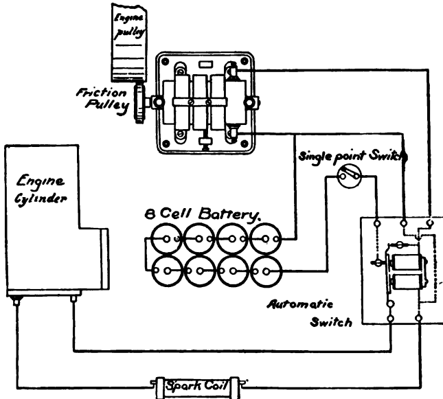
FIG. 338.—A Primary Spark Ignition Circuit, containing a magneto-generator, an 8-cell chemical battery, and an automatic cut-off or relay. The chemical battery is used to supply the current for producing the spark until the magneto-generator has attained its required speed. At that point the current from the generator passing through the coil of the automatic switch is sufficiently strong to cause the magnets of the relay to attract their armature and cut the circuit of the chemical battery. This circuit may also be cut out at any time desired with the single point hand switch.
